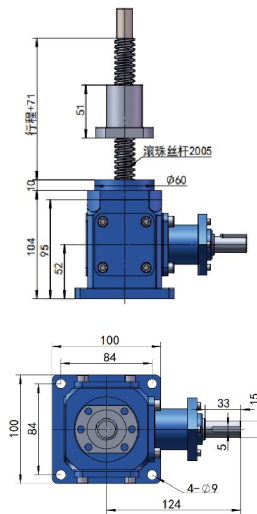
2A螺母在上 2A Upright rotating screw
