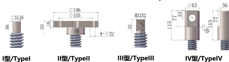
丝杆头部可选/Screw head optional
