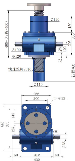
1A Upright translating ball screw optional
