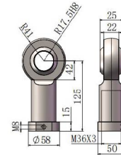
R型结构/Type R structure
