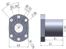
Type 2 Ball screw nut
