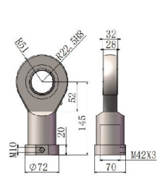
R型结构/Type R structure
