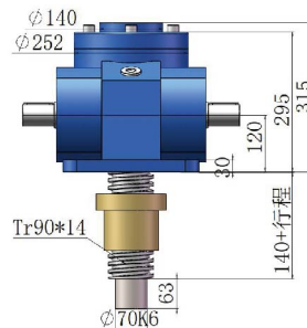
丝杆头部可选/Screw head optional
