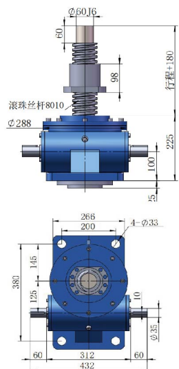
2A Upright rotating screw
