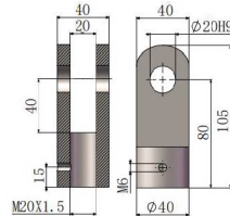
叉销端FO Fork Pin End FO
