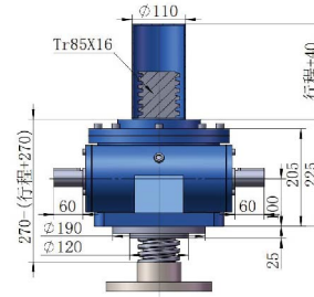
丝杆头部可选/Screw head optional
