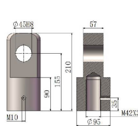
R型结构/Type R structure
