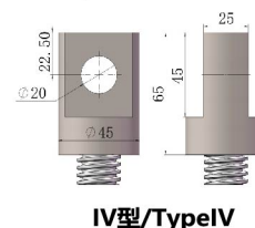
滚珠丝杆头部可选/Ball screw head optional
