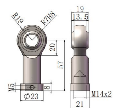
球型铰接TS Spherical joint TS
