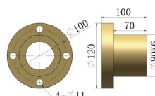
2型丝杆螺母/Type 2 screw nut
