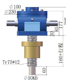
F螺母在下 F Inverted rotating screw
