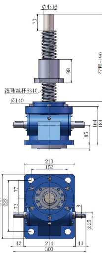
2A螺母在上 2A Upright rotating screw
