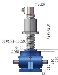
2A螺母在上 2A Upright rotating screw
