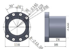
2型滚珠丝杆螺母 Type 2 ball screw nut
