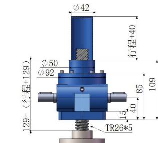
丝杆头部可选/Screw head optional
