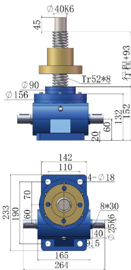
轴指向/Shaft direction
