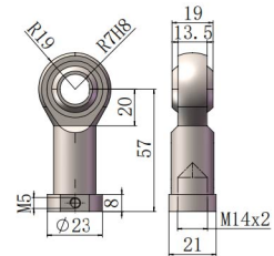
R型结构/Type R structure
