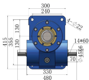
轴指向/Shaft direction
