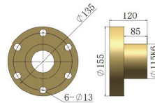
2型丝杆螺母/Type 2 screw nut
